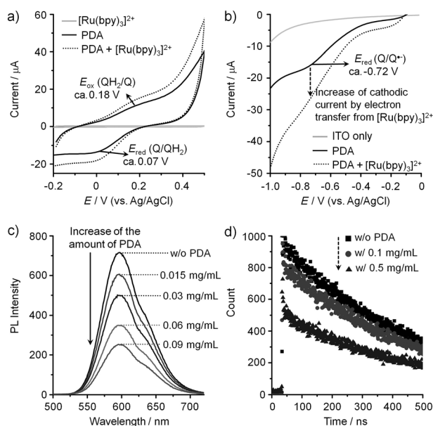
Figure 3. Electron delivery from [\text{Ru}(\text{bpy})_3]^{2+} to PDA. a) Cyclic and b) linear-sweep voltammogram of a [\text{Ru}(\text{bpy})_3]^{2+} -containing phosphate buffer (10 mM, pH 8.0) in the absence and presence of PDA. The potential was scanned at 100 \text{ mV s}^{-1} . The redox peaks at 0.07 and 0.18 V (vs. Ag/AgCl) in Figure 3a correspond to the reduction and oxidation of PDA, respectively. In addition, the cathodic peak at -0.72 \text{ V} is the reduction potential of the quinone group of PDA to form radical quinone anions, according to the literature [20]. c) Changes in the emission spectrum of [\text{Ru}(\text{bpy})_3]^{2+} in the presence of various amounts of PDA. d) Photoluminescence decay profiles of [\text{Ru}(\text{bpy})_3]^{2+} in the presence of PDA at different concentrations. w/ = with, w/o = without.
