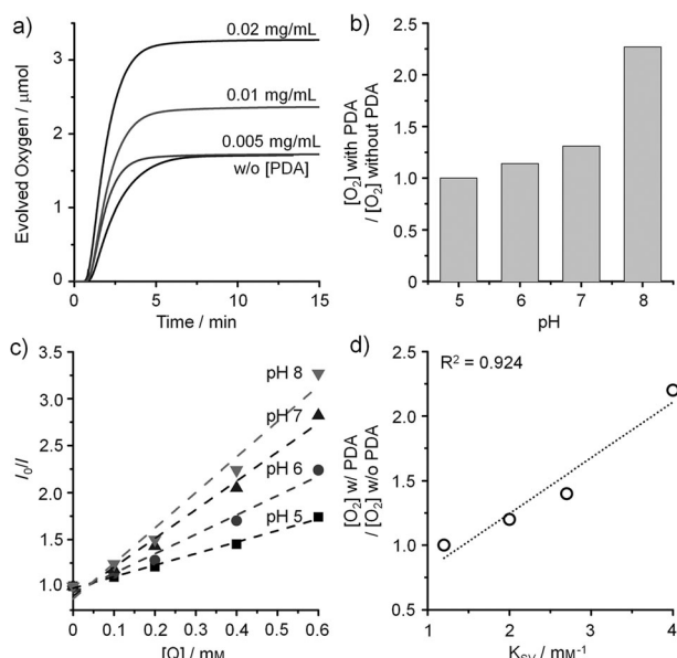
Figure 4. a) Time profiles of oxygen evolution for 0.01 mM Co-Pi with 0.25 mM [\text{Ru}(\text{bpy})_3]^{2+} and varying concentrations of PDA in a phosphate buffer at pH 8.0 containing 5 mM sodium persulfate. b) Ratio of the amounts of evolved oxygen with and without PDA at different pH values. c) Stern–Volmer plot for [\text{Ru}(\text{bpy})_3]^{2+} in the presence of semiquinone groups of PDA at different concentrations. The concentrations of the semiquinone groups of PDA were determined by elemental analysis. Slopes of Stern–Volmer plot were substantially increased with an increasing pH value. d) Plot showing the relationship between catalytic activity and the Stern–Volmer coefficient ( K_{\text{SV}} ). Catalytic activity was defined as a ratio of oxygen evolution with PDA to that without PDA.
